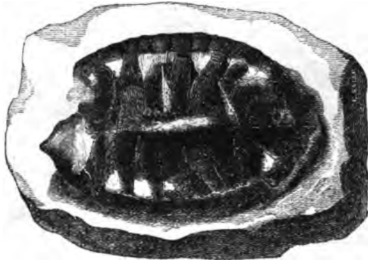
CHELONIA BENSTEDL. (Chalk.)
